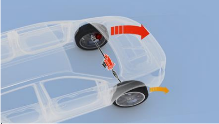
Mekaaninen kitkalukko Mechanical Limited Slip Differential (m-LSD)
